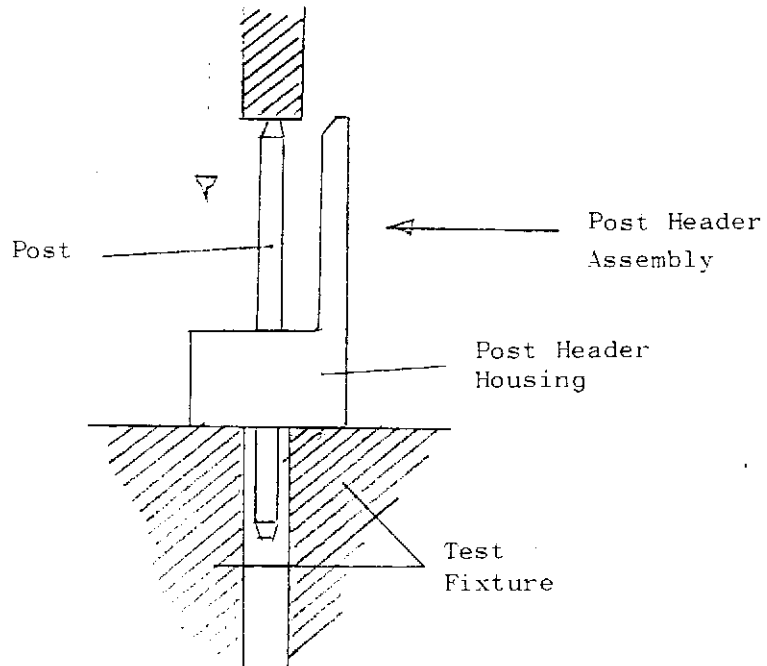
Fig. 3 Post Retention Force Measuring Method
